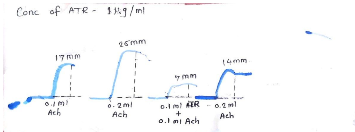
Figure 1:- Effect of ATROPIN(1 \mu g/ml) on DRC of Ach by using isolated chicken ileum preparation.
