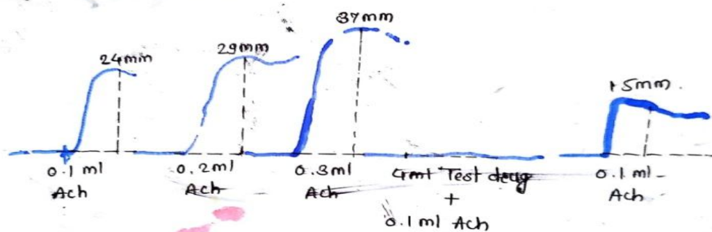
Figure 6:- Effect of test drug 800mg/ml on DRC of Ach by using isolated chicken ileum preparation .
