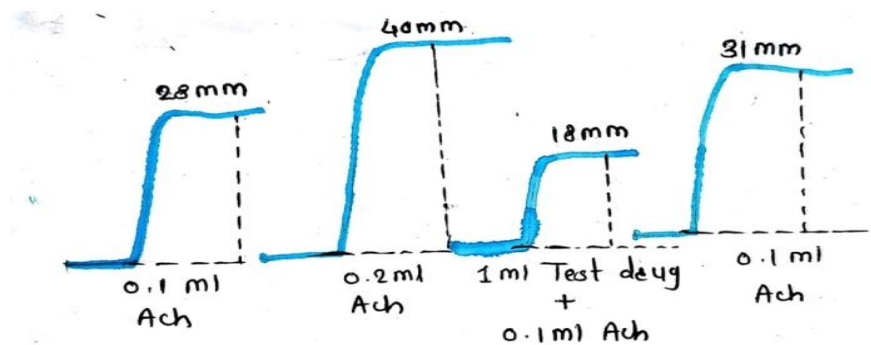
Figure 3 :- Effect of Test drug 9200mg/ml) on DRC of Ach by using isolated chicken ileum preparation.
