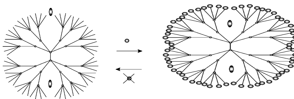
Figure 2: Dendritic box, encapsulating guest drug molecules.
