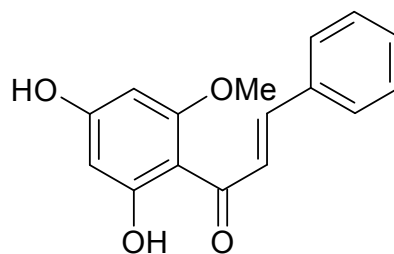
Figure 1: Cardamonin
